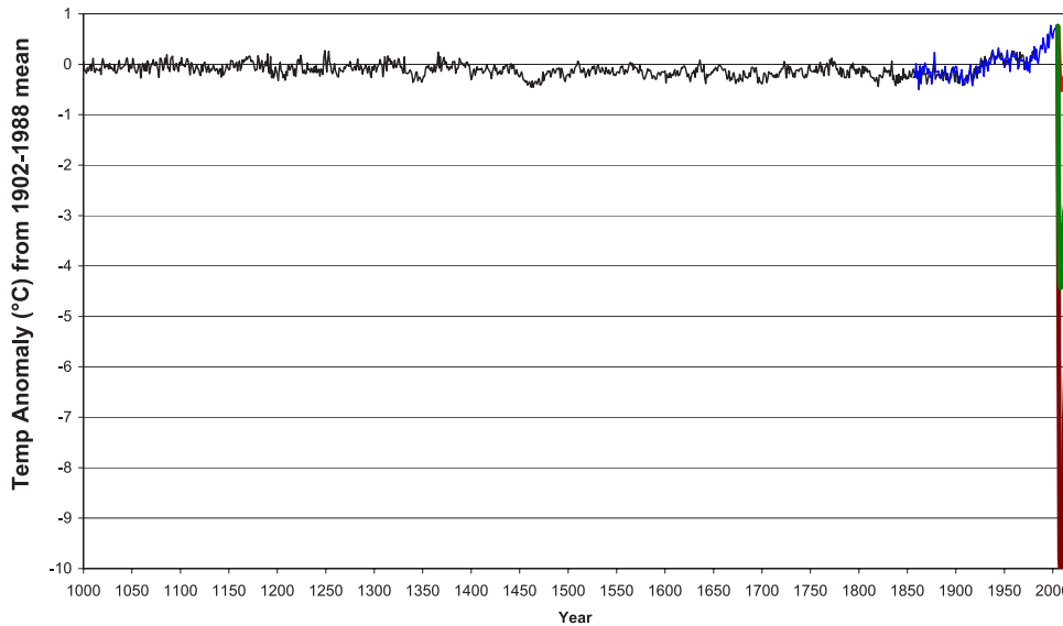
Figure 9. Northern Hemisphere average surface air temperature change from 5 Tg (red), 50 Tg (green), and 150 Tg (brown) cases in the context of the climate change of the past 1000 years. The “hockey stick” nature of the curve is barely discernible when plotted on this scale. Black curve is from Mann et al. [1999], and the blue curve is from the latest data from the Climatic Research Unit website ( http://www.cru.uea.ac.uk/cru/data/temperature/ ).
